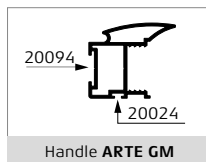
Handle ARTE GM
