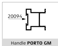
Handle PORTO GM
